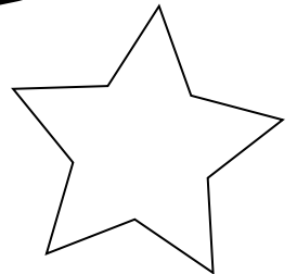
Mercure
